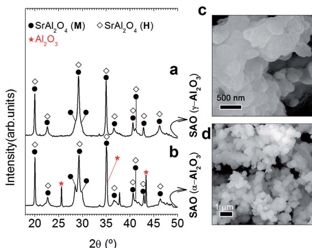
Fig. 2 Role of the alumina precursor excess in structural and micro-structural characterization: XRD patterns of \text{SrAl}_2\text{O}_4 : Eu, Dy (SAO) phosphor employing two alumina precursors: \gamma\text{-Al}_2\text{O}_3 (a) and \alpha\text{-Al}_2\text{O}_3 (b) and an \text{Al}_2\text{O}_3 /SrO ratio of 2. The symbols highlight \text{SrAl}_2\text{O}_4 (monoclinic, black circle), \text{SrAl}_2\text{O}_4 (hexagonal, black-open diamonds), and \text{Al}_2\text{O}_3 (red star). Detail micrograph of \text{SrAl}_2\text{O}_4 : Eu, Dy (SAO) phosphor using as precursors \gamma\text{-Al}_2\text{O}_3 (c) and \alpha\text{-Al}_2\text{O}_3 (d).
