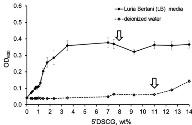
Fig. 2 Optical density ( OD_{600} ) measurements versus the concentrations of 5'DSCG in deionized water and in LB media. Arrows indicate the concentrations at which the liquid crystal (LC) phase forms.
