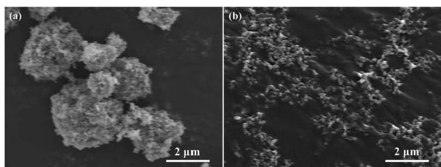
Fig. 8 SEM images of (a) TiO 2 nanoparticles and (b) BAD/nano-TiO 2 complex.
