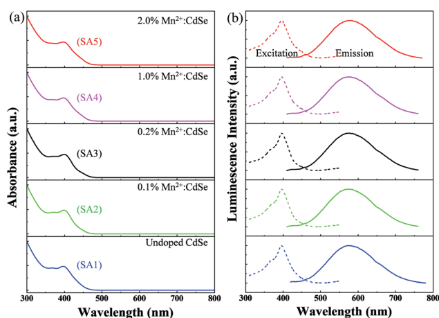
Fig. 2 (a) Normalized UV-vis absorption and (b) PL excitation (dashed line) and emission (solid line) spectra of all five CdSe QDs sample with various \text{Mn}^{2+} -dopant ion concentration synthesized in aqueous medium.
