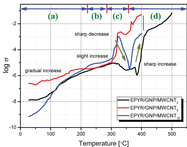
Fig. 5 In situ electrical conductivity measurements for pure EPYR and its corresponding EPYR/GNP/MWCNT 2–10 composite materials, at a heating rate of 10° min -1 .
