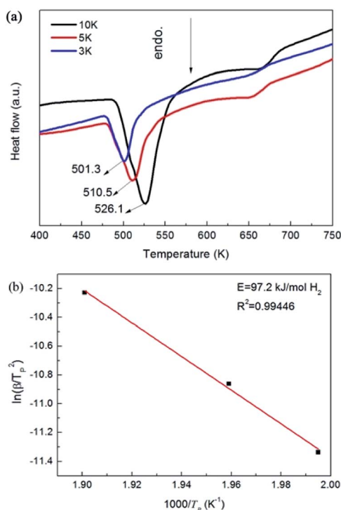
Fig. 8 DSC profiles of the \text{Mg}-\text{Ni}(\text{Fe})-\text{H} sample measured at different heating rates (a) and the corresponding \ln(\beta/T_p^2)-1000/T_p plot (b).
