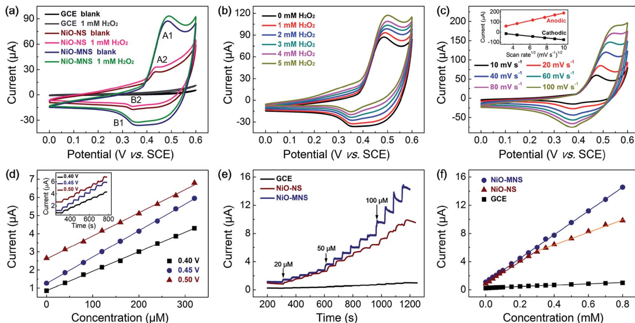
Fig. 4 (a) CV curves of the bare GCE, NiO-NS and NiO-MNS electrodes with and without 1 mM \text{H}_2\text{O}_2 . (b) CV curves of the NiO-MNS electrode with different \text{H}_2\text{O}_2 concentrations at a scan rate of 20 \text{ mV s}^{-1} . (c) CV curves the NiO-MNS electrode with different scan rates, and the inset in (c) shows the \text{Ni(II/III)} redox peak currents at different scan rates. (d) Linear relationship between the response current and the \text{H}_2\text{O}_2 concentration, and the inset in (d) shows chronoamperometric response of NiO-MNS towards the step injection of 40 \mu\text{M} \text{H}_2\text{O}_2 solution at different potentials. (e) Chronoamperometric response of GCE, NiO-NS and NiO-MNS towards the injection of hydrogen peroxide at 0.45 \text{ V} . (f) Linear relationship between the response current and the \text{H}_2\text{O}_2 concentration. Geometric loading of NiO-NS and NiO-MNS on the GCE is 425 \mu\text{g cm}^{-2} .
