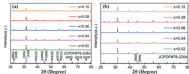
Fig. 2 XRD patterns of (a) \text{BaTiO}_3\text{:xEu}^{3+} ; (b) \text{BaTiO}_3\text{:xDy}^{3+} , x = 0.02\text{--}0.10 , prepared at 750^\circ\text{C} for 4 hours.
