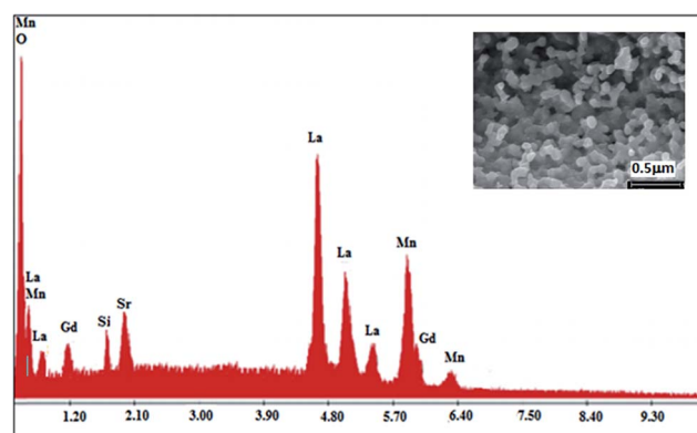
Fig. 1 EDX spectra of the \text{La}_{0.6}\text{Gd}_{0.1}\text{Sr}_{0.3}\text{Mn}_{0.75}\text{Si}_{0.25}\text{O}_3 compound. The inset shows a typical scanning electron microscopy (SEM) image.
