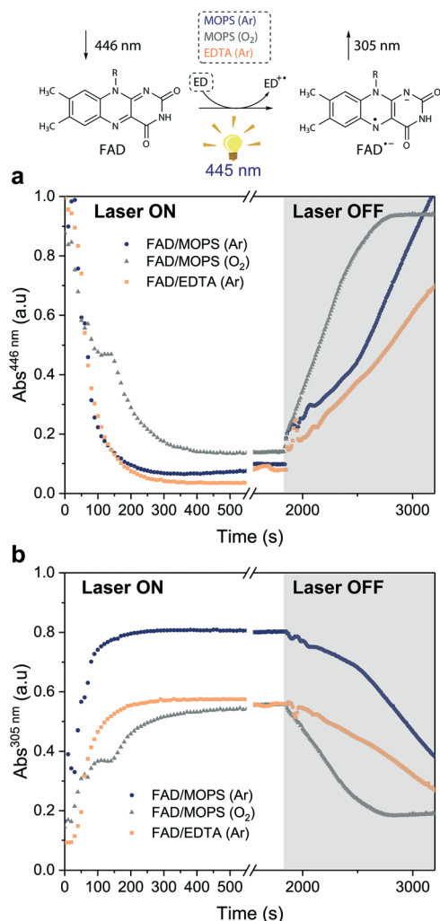
Fig. 5 Steady-state absorption measurements under light excitation ( \lambda_{\text{EX}} = 445 nm). Kinetic traces extracted from the absorption spectra of the reactions between: (i) FAD and MOPS in the absence (dark blue circles) and in the presence of oxygen (gray triangles) and (ii) FAD and EDTA (orange squares) in Tris-HCl. Kinetic traces at (a) 446 nm (FAD ground-state) and (b) 305 nm (FAD anionic semiquinone). The laser was switched off after 30 min of irradiation (gray region).
