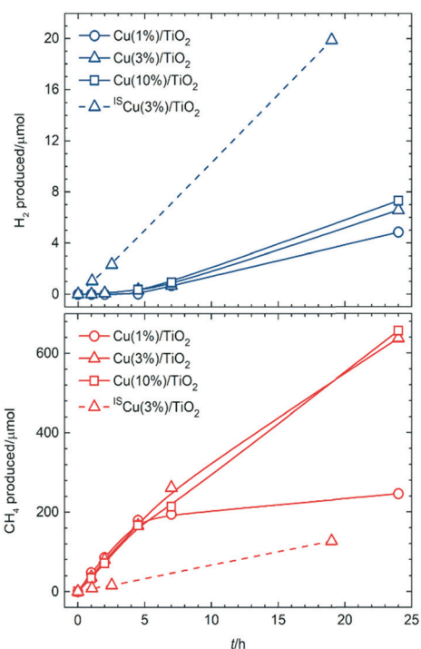
Fig. 2 Amounts of \text{H}_2 and \text{CH}_4 formed upon simulated sunlight irradiation of aqueous acetic acid on conventional \text{Cu}(X\%)/\text{TiO}_2 and in situ ( ^{15}\text{Cu}(X\%)/\text{TiO}_2 ) photocatalysts as a function of increasing irradiation times. Reaction conditions as in Fig. 1.
