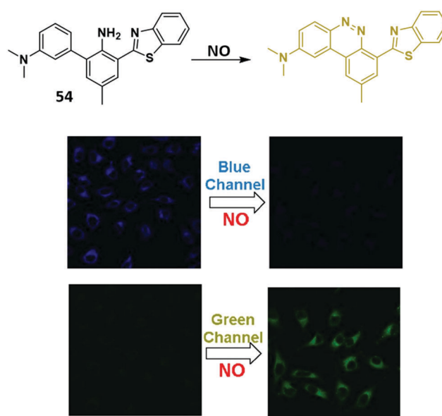
Scheme 50 An ES IPT fluorescent probe 54 for the ratiometric detection of NO via formation of a benzo[c]cinnoline derivative. Measurement conditions: PBS buffer (1.0 mM, pH = 7.4). Reproduced with permission from ( Sens. Actuators, B , 2018, 259 , 347–353). Copyright (2018) Elsevier.
