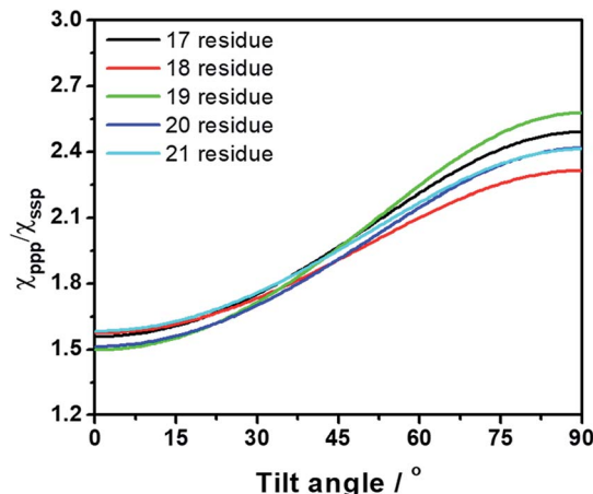
Fig. 3 Dependence of the tilt angle on the measured SFG signal strength \chi_{ppp}/\chi_{ssp} ratio for several different lengths of alpha-helical peptide (17–21 residues).
