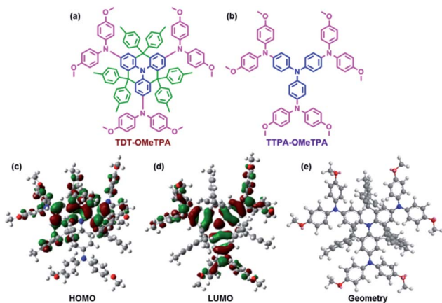
Fig. 1 Molecular structures of (a) TDT-OMeTPA and (b) TTPA-OMeTPA. The (c) HOMO, (d) LUMO and (e) optimized molecular conformation of TDT-OMeTPA obtained from DFT calculations.
