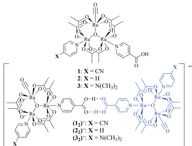
Fig. 1 (top) Oxo-centered triruthenium cluster of the type [\text{Ru}_3(\mu_3\text{-O})(\text{OAc})_6(\text{CO})(\text{L}_1)(\text{ina})]^- where \text{L}_1 = 4\text{-cyanopyridine (cpy, 1)} , \text{pyridine (py, 2)} , or 4\text{-dimethylaminopyridine (dmap, 3)} and \text{ina} = \text{isonicotinic acid} . (bottom) Dimerization interaction upon a one electron reduction to generate the hydrogen-bonded, mixed-valent ions, (1_2)^- , (2_2)^- , (3_2)^- .
