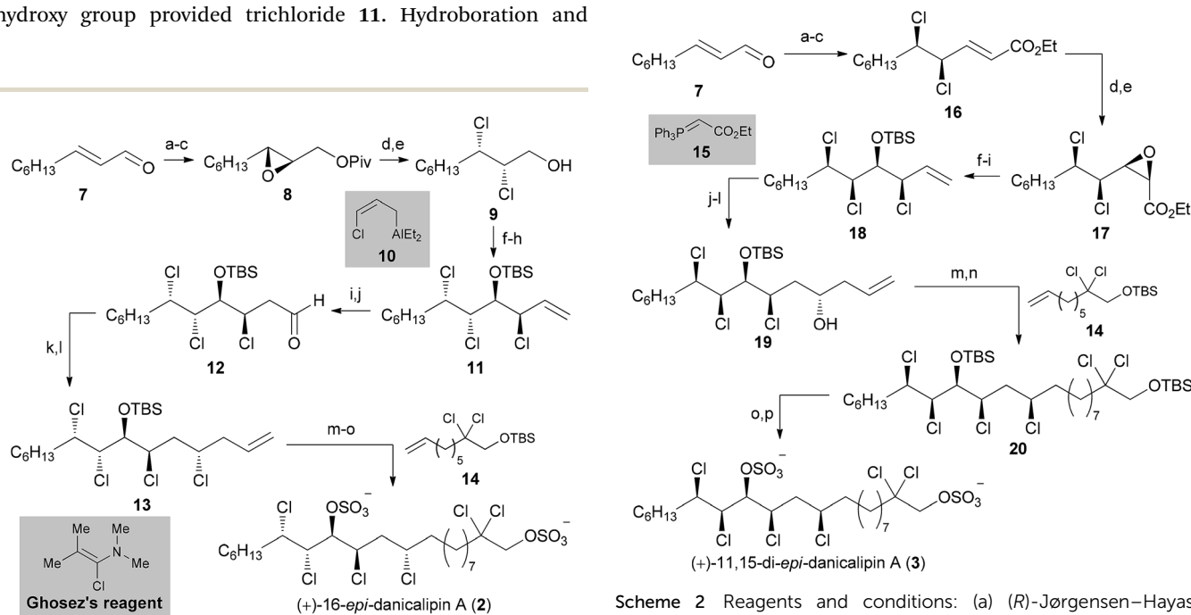
Scheme 1 Reagents and conditions: (a) ( S )-Jørgensen–Hayashi catalyst (10 mol%), H 2 O 2 , CH 2 Cl 2 , r.t., e.r. > 20 : 1; (b) NaBH 4 , MeOH, 0 °C, 62% over 2 steps; (c) PivCl, pyridine, CH 2 Cl 2 , r.t., 82%; (d) PPh 3 , NCS, toluene, 90 °C; (e) (iBu) 2 AlH, CH 2 Cl 2 , –78 °C, 78% over 2 steps; (f) DMP, NaHCO 3 , CH 2 Cl 2 , r.t.; (g) 10 , THF, –78 °C, d.r. > 6 : 1; (h) TBSOTf, Et 3 N, CH 2 Cl 2 , r.t., 47% over 3 steps; (i) Cy 2 BH, THF, 0 °C, then NaBO 3 ·4H 2 O, r.t., 69%; (j) DMP, CH 2 Cl 2 , r.t.; (k) (+)-Ipc 2 B(allyl), THF, –100 °C to r.t., 83% over 2 steps, d.r. > 5 : 1; (l) Ghosez's reagent, CHCl 3 , then Et 3 N, r.t., 86%; (m) 14 (3 equiv.), Grubbs II (10 mol%), CH 2 Cl 2 , 45 °C, then PtO 2 (10 mol%), H 2 (1 atm), r.t., 90%; (n) AcCl, MeOH, 80 °C, 84%; (o) SO 3 ·pyridine, THF, r.t., 87%.
