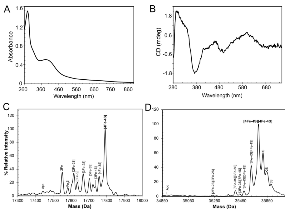
Fig. 2 Characterization of the RirA iron–sulfur cluster. (A) UV-visible absorbance and (B) CD spectra of reconstituted RirA (371 μM [4Fe–4S] RirA) in buffer B. Pathlength 1 mm. (C) and (D) Positive ion mode ESI-MS deconvoluted spectra of RirA (30 μM in cluster in 250 mM ammonium acetate pH 7.32) under non-denaturing conditions in the monomer (C) and dimer (D) mass regions.
