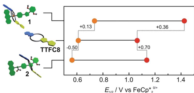
Fig. 5 Correlation diagram of half-wave potentials for charged [2]rotaxane 1 , macrocycle TTFc8 and neutral, acetylated [2]rotaxane 2 . Half-wave potentials were determined by cyclic voltammetry measurements in \text{CH}_2\text{Cl}_2 against \text{Fe}(\text{Cp}^*)_2^{0/+} with a 1 \text{ mM} analyte concentration at a scan rate of 100 \text{ mV s}^{-1} with tetrabutylammonium \text{BARF}_{24} ( 0.1 \text{ M} ) as the electrolyte.
