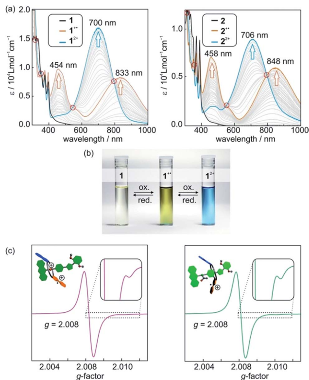
Fig. 4 (a) Photometric titrations of [2]rotaxanes 1 (left) and 2 (right) with \text{Fe}(\text{ClO}_4)_3 as the oxidant ( 50 \mu\text{M} rotaxane solutions in \text{CH}_2\text{Cl}_2 ). The isosbestic points indicate two clean one-electron oxidations and are marked with red circles. (b) Photographs of 1 \text{ mM} \text{CH}_2\text{Cl}_2 solutions of [2]rotaxane 1 before oxidation and after the addition of one or two equivalents of oxidant \text{Fe}(\text{ClO}_4)_3 . (c) X-band EPR spectra of \text{CH}_2\text{Cl}_2 solutions ( 0.1 \text{ mM} ) of [2]rotaxanes 1^{\bullet+} (left) and 2^{\bullet 2+} (right) after addition of one equivalent of \text{Fe}(\text{ClO}_4)_3 .
