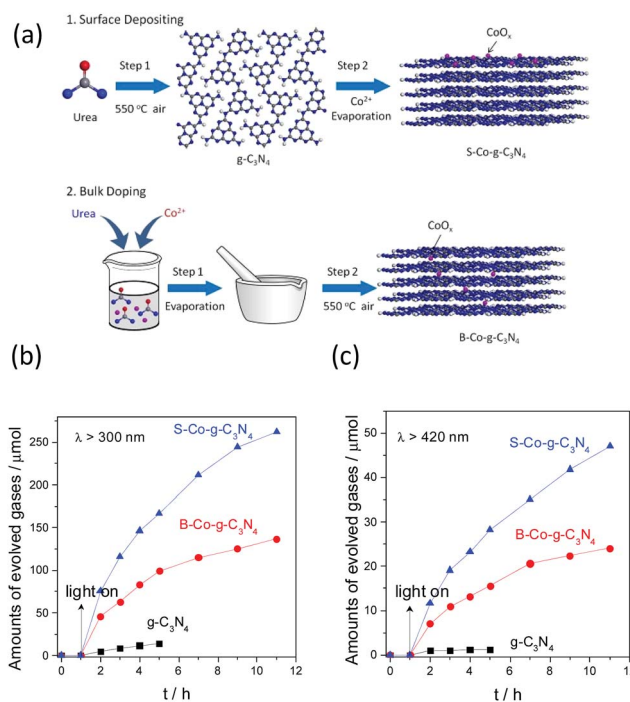
Fig. 11 (a) Schematic illustration of surface deposition and bulk doping modification of \text{g-C}_3\text{N}_4 . Photocatalytic water oxidation activities of the \text{g-C}_3\text{N}_4 , B-Co-g- \text{C}_3\text{N}_4 and S-Co-g- \text{C}_3\text{N}_4 samples under (b) UV ( \lambda > 300 \text{ nm} ) and (c) visible light ( \lambda > 420 \text{ nm} ) irradiation. Reprinted with permission from ref. 107. Copyright 2016, American Chemical Society.
