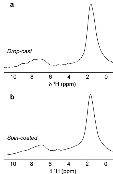
Fig. 7 ^1\text{H} MAS NMR spectra of (a) drop-cast and (b) spin-coated films of DPP-DDT on crushed glass substrates recorded at 18.8 T and a MAS frequency of 60 kHz.
