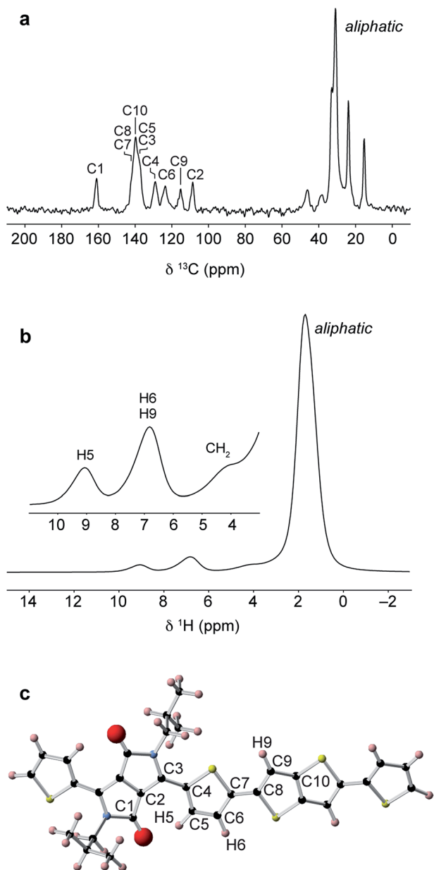
Fig. 4 (a) {}^1\text{H} - {}^{13}\text{C} CPMAS and (b) {}^1\text{H} MAS NMR spectra of DPP-DTT bulk polymer. Spectra were recorded at magnetic field strengths of (a) 9.4 and (b) 18.8 T, and MAS frequencies of (a) 12.5 and (b) 60 kHz. (c) DFT-optimized polymer fragment used for NMR chemical shift calculations.
