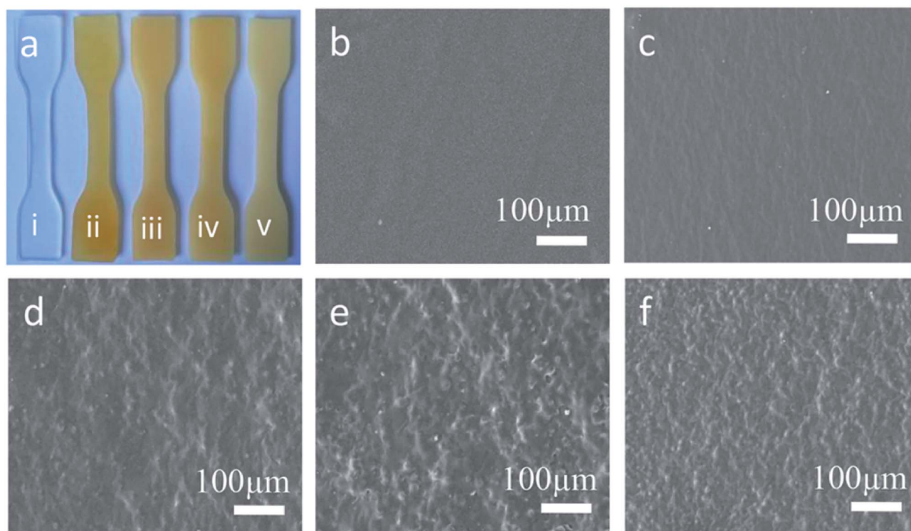
Fig. 5 Morphologies and microstructures of RTV silicone rubbers. (a) Photo of (i) SRER-1, (ii) SRER-2, (iii) SRER-3, (iv) SRER-4, (v) SRER-5. SEM images of (b) SRER-1, (c) SRER-2, (d) SRER-3, (e) SRER-4, (f) SRER-5.
