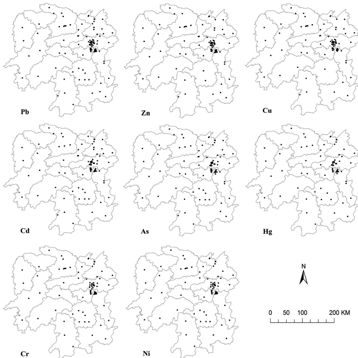
Fig. 1 Distribution of sampling sites of soil Pb, Zn, Cu, Cd, As, Hg, Cr, and Ni in Hunan province.
