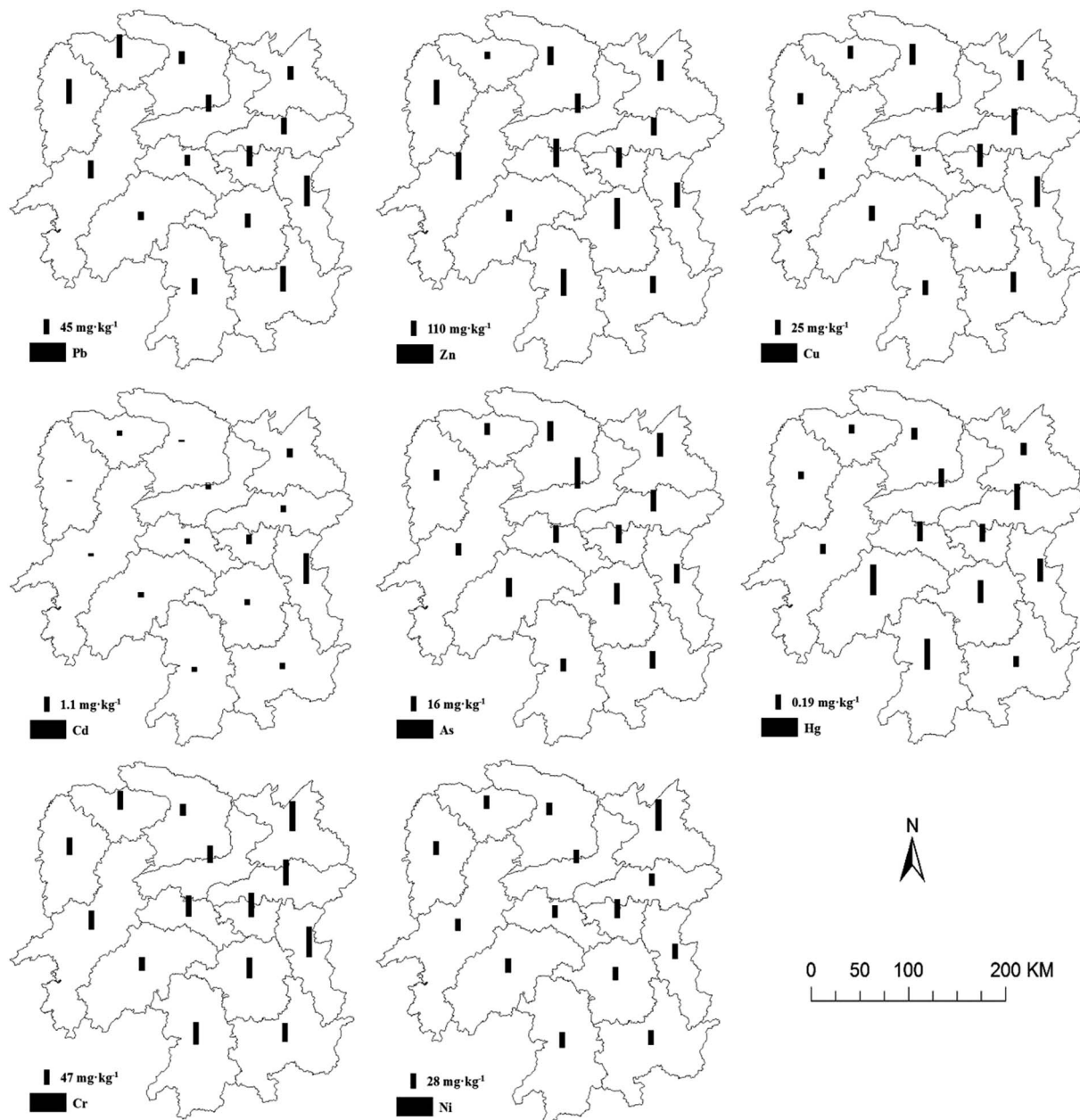
Fig. 2 Contents of 8 heavy metal in soil, Hunan province.
