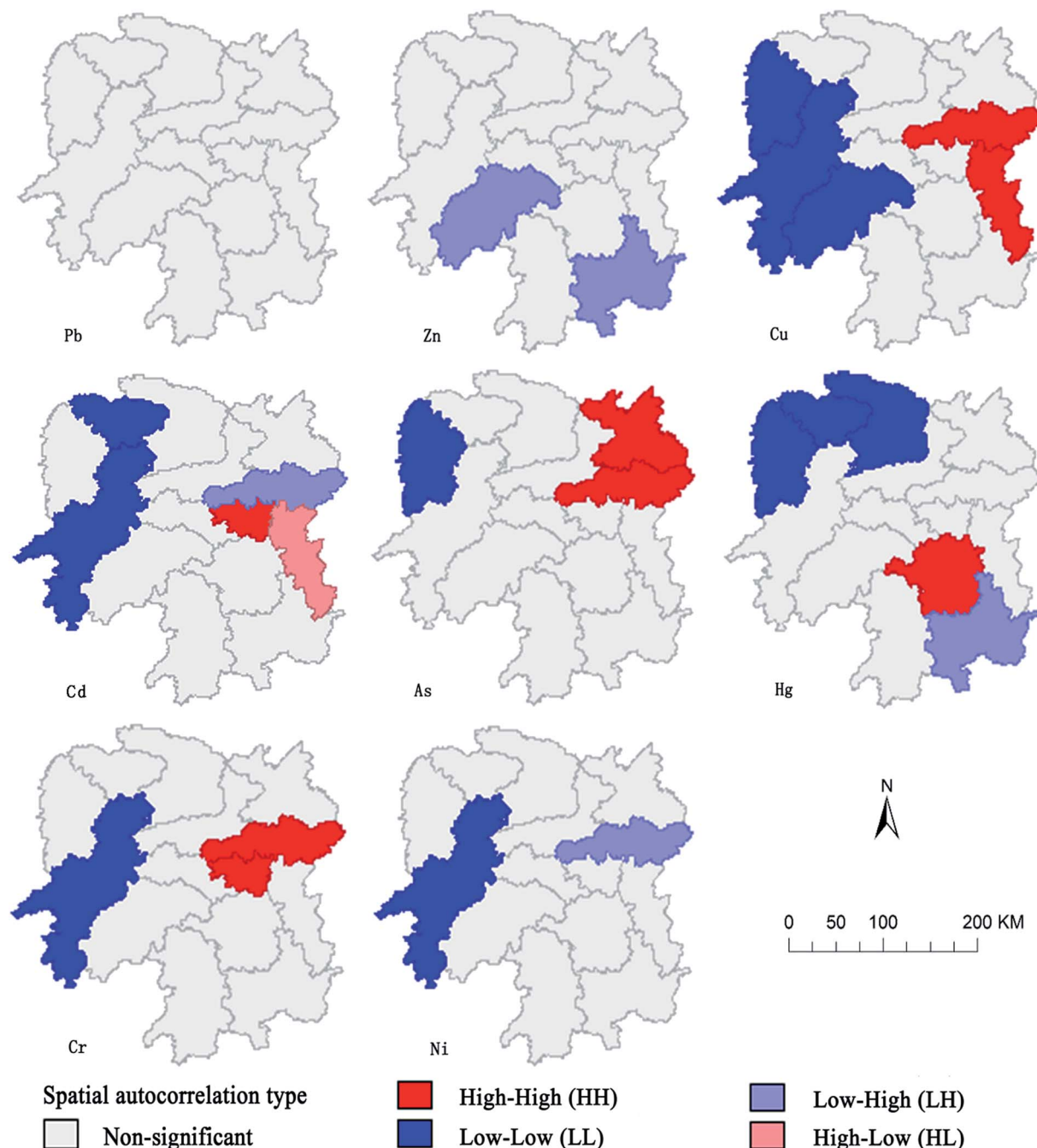
Fig. 3 LISA map of ESR of the 8 soil heavy metals in Hunan province.
