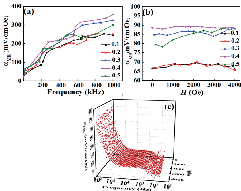
Fig. 8 Magnetoelectric coefficient \alpha_{ME} for various applied (a) frequencies and (b) dc magnetic field of the BT-BFO- x LFO ( x = 0.1-0.5 ) ceramics sintered at 1300 °C and (c) 3D image of BT-BFO-0.4LFO ceramic.
