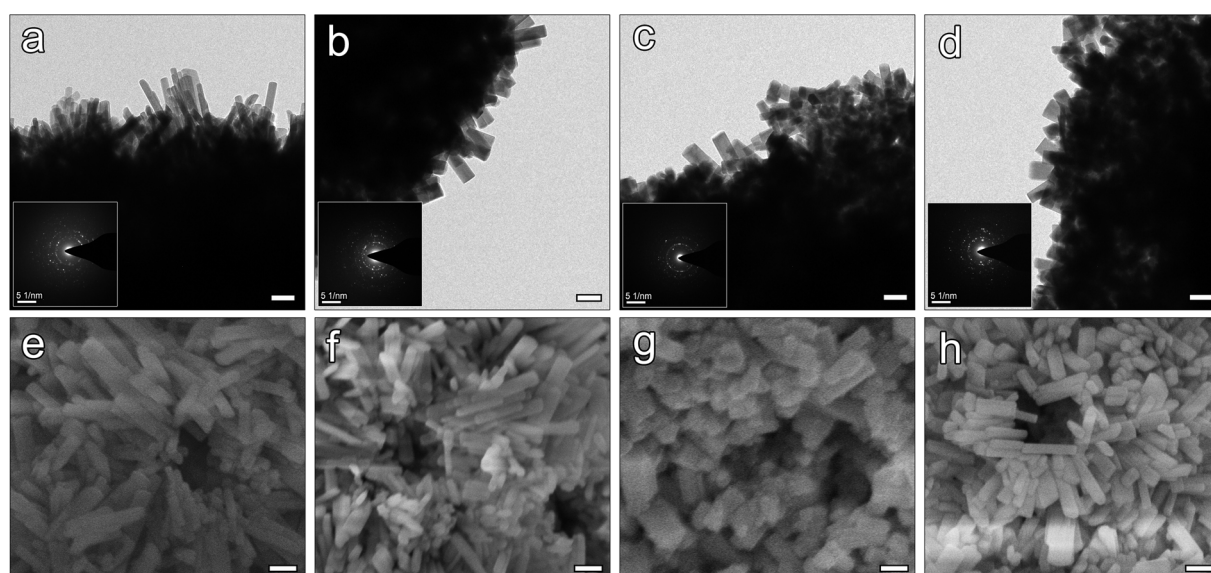
Fig. 3 Magnified TEM (scale bar = 100 nm) images with corresponding SAED patterns (scale bar = 5 1/\text{nm} ) showing the nano-sized HAP crystals of A-CHAM (a), B-CHAM (b), C-CHAM (c) and D-CHAM (d). Magnified SEM (scale bar = 100 nm) images showing the morphology of the HAP crystals and mesoporous structures of A-CHAM (e), B-CHAM (f), C-CHAM (g) and D-CHAM (h).
