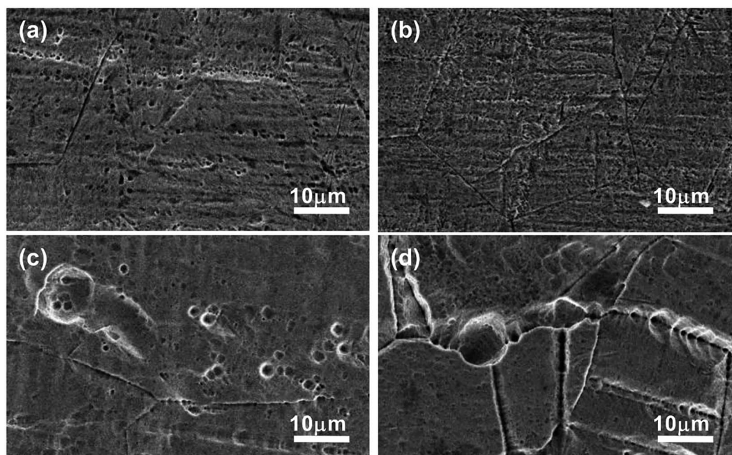
Fig. 8 SEM of the surfaces of stainless steel after immersion in (a) IL, (b) IL + MO, (c) IL + MO + \text{H}_2\text{O} , (d) IL + MO + \text{H}_2\text{O}_2 at 45 ^\circ\text{C} for 14 days.
