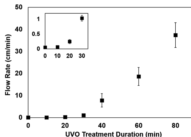
Fig. 6 Capillary flow rate as a function of UVO treatment duration for PMMA microchannels. Inset shows magnified view of the data points at lower (<40 min) UVO exposure times. Each data point represents the mean \pm SD of three measurements.
