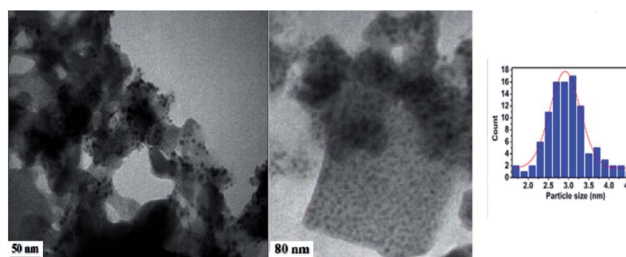
Fig. 3 TEM micrograph of the PdNPs/Cu 2 (BDC) 2 DABCO.
