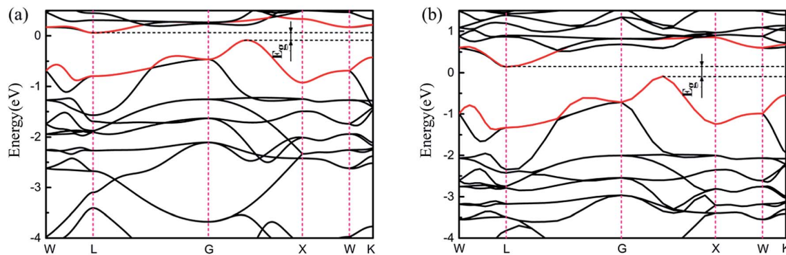
Fig. 7 (a) and (b) are the band structure of the \text{Ce}_1\text{Ni}_{1-p} phase using PBE and HSE06 functional, respectively.
