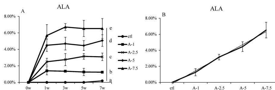
Fig. 1 ALA content in blood of different ALA levels groups. (A) Percent composition of ALA in the blood samples after seven weeks for the five diet groups. (B) The linear relationship between ALA levels in the whole blood and dietary ALA content. Bars labeled (7w) with different letters are significantly different from each other ( p < 0.05 ).
