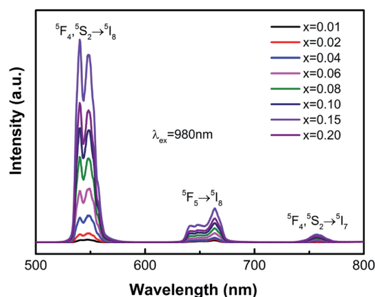
Fig. 2 Upconversion emission ( \lambda_{\text{ex}} = 980 nm) spectra of \text{ZnWO}_4:0.01\text{Ho}^{3+}/x\text{Yb}^{3+} phosphors at room temperature.
