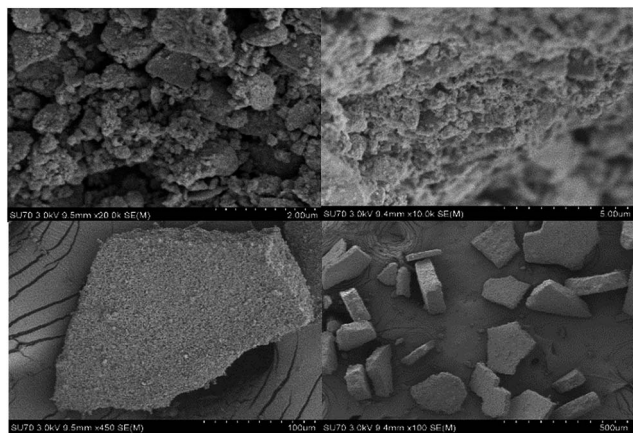
Fig. 7 SEM images of Al/Fe oxide RNGO after its fifth run in the recyclability experiment.
