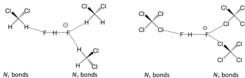
Fig. 12 The scheme introducing the numbers N_1 and N_2 of solvent molecules interacting with FHF - anion. Left: FHF - in CH 2 Cl 2 ( r' < 2.5 Å; 150^\circ < \beta < 180^\circ ); right: FHF - in CCl 4 ( r' < 3.1 Å; 150^\circ < \beta < 180^\circ ). For the definitions of r' and \beta see Fig. 8, top.
