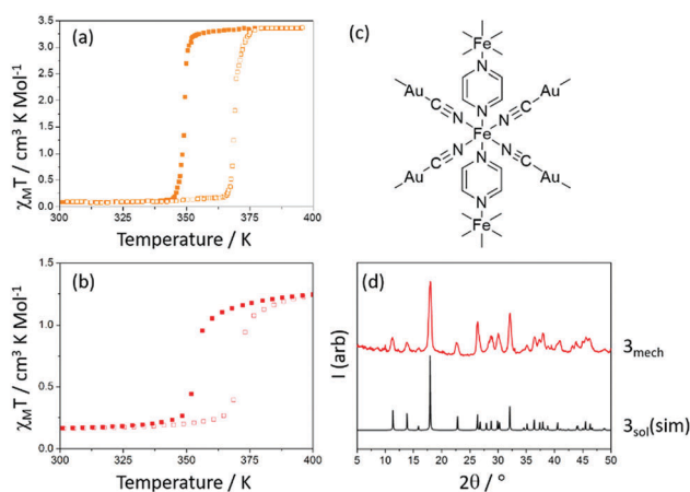
Fig. 4 (a) \chi_M T versus T for 3 sol adapted from ref. 18 (b) \chi_M T versus T for 3 mech (c) structure of 3 and (d) PXRD of complex 3 (simulated from single crystal data 20 ), and 3 mech .
