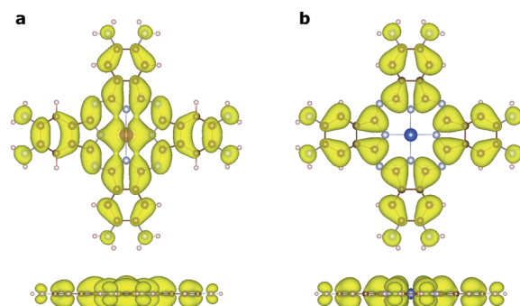
Fig. 6 Visualization of the highest occupied molecular orbitals (HOMOs) of octaamino-MPc molecules by charge density isosurfaces. (a) Strong hybridization is evident between the d_{\pi} orbitals of Mn and the \pi orbitals of the ligand in octaamino-MnPc. (b) No contribution is observed from the metal d orbitals in the HOMO charge density isosurface of octaamino-MPc, where M is Cr, Fe, Co, Ni, Cu, or Zn. Both top and side views of the charge density isosurfaces ( \rho = 0.001 electrons per \text{\AA}^3 ) are shown.
