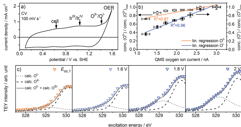
Fig. 2 (a) Cyclic voltammogram, (b) normalized O^{1-} and O^{2-} concentrations over QMS oxygen ion current, and (c) zoomed and fitted low excitation energy regions of O K-edges recorded in the three-electrode cell (indicated potentials vs. SHE, ring current = 60 mA, p = 0.3 Pa, 0.1 M H_2SO_4 ).
