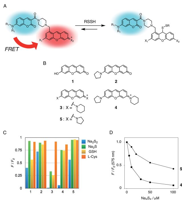
Fig. 1 (A) Mechanism of the FRET-based ratiometric fluorescence sensing of hydropersulfide. (B) Structure of the xanthenone derivatives. (C) Fluorescence quenching efficiency ( F/F_0 ) of 1–5 upon addition of Na_2S_2 (50 \mu M), Na_2S (50 \mu M), GSH (5 mM), and L-Cys (1 mM). The data were measured 10 min after addition of the thiol compounds. Measurement conditions: [probe] = 5 \mu M in 50 mM HEPES, 10 mM NaCl, 1 mM MgSO_4 , pH 7.4, 25 ^{\circ}C . \lambda_{ex} = 480 nm ( 1 ), 500 nm ( 2 ), 530 nm ( 3 , 4 , 5 ). (D) Fluorescence titration profile of 4 (■) and 5 (●) upon addition of Na_2S_2 (0–100 \mu M). Measurement conditions: [probe] = 5 \mu M in 50 mM HEPES, 10 mM NaCl, 1 mM MgSO_4 , pH 7.4, 25 ^{\circ}C . \lambda_{ex} = 530 nm.
