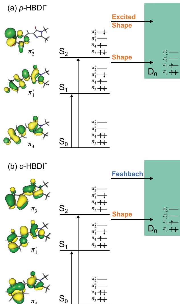
Fig. 6 Energy level diagram of (a) p -HBBDI − and (b) o -HBBDI − in which possible excitations and subsequent detachment processes are indicated (note that it is only the vibrationally excited states of S 1 lying in the D 0 continuum that have shape resonance character). S 1 and S 2 refer to the first two excited states selected in Table 2. The HOMO is \pi_4 and the LUMO is \pi_1^* . Alongside are the Hartree–Fock molecular orbitals that are involved in the excitations. For op -DHBBDI − , a similar scheme applies as for p -HBBDI − except the excited state resonance is S 3 (Table 2).
