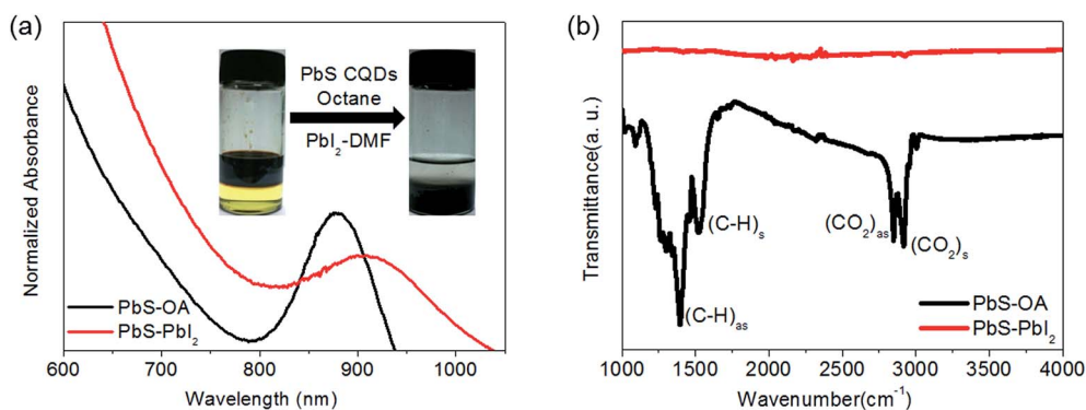
Fig. 3 (a) Absorption spectra of the PbS QDs before (black) and after the \text{PbI}_2 treatment (red). The inset shows the solution-processed phase transfer process. (b) FTIR spectra of PbS-OA and PbS- \text{PbI}_2 .
