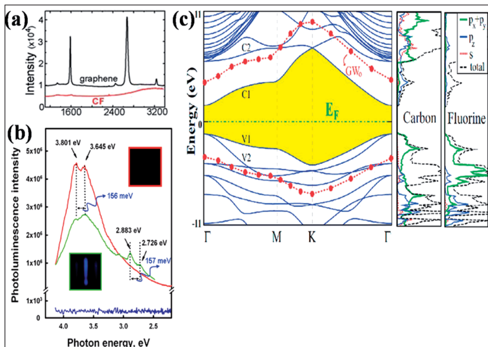
Fig. 11 (a) Raman spectra comparing graphene on SiO 2 and CF formed on SiO 2 . Reproduced with permission. 129 © 2010 American Chemical Society. (b) Room temperature recorded photoluminescence emission (excitation at 290 nm (4.275 eV)) of graphene shown in blue (with no PL peak) and fluorographene (green, fluorination for 1 day; red, fluorination for 5 days). Reproduced with permission from ref. 131. © 2011 American Chemical Society. (c) Band structure and orbital PDOS together with total DOS of fluorographene. The LDA recorded band gap is shaded, and the Fermi level is set to zero energy. After GW_0 correction, the conduction and valence band edges are represented by filled (red) circles. Reproduced with permission. 132 © 2011 American Physical Society.
