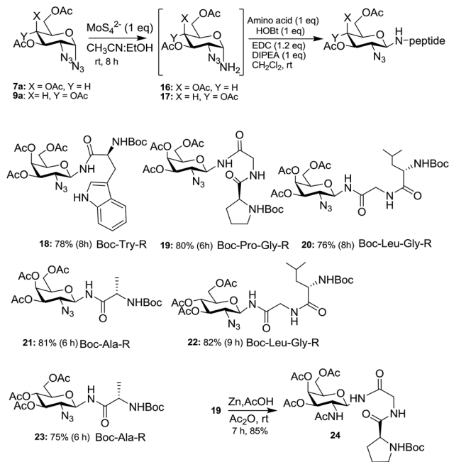
Scheme 5 Selective reduction of 1,2-diazides and synthesis of \beta - N -glycopeptides.
