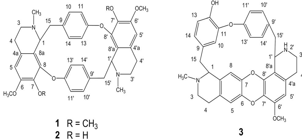
Fig. 1 Chemical structures of cycleanine (1), isochondodendrine (2) and 2'-norcoculine (3) from T. subcordata .
