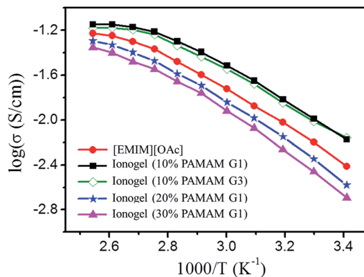
Fig. 5 Temperature dependence of the ionic conductivities of neat [EMIM][OAc] and ionogels shown in the Arrhenius convention.
