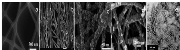
Fig. 1 SEM images of various types of CNF synthesized from cotton (a) natural electrospun CNF 56 (b) aligned CNF (scale bar 1 μm) 54 (c): CdS functionalized CNF 53 (d): CeO 2 functionalized CNF 56 (e): CNF prepared by acid hydrolysis 52 (adopted with permission).
