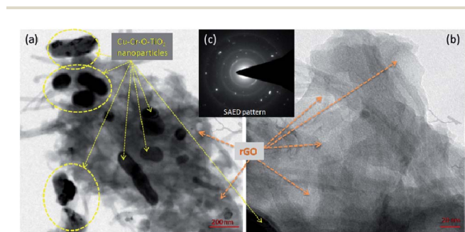
Fig. 5 TEM images of synthesized catalyst at two different magnifications (a) 200 nm and (b) 20 nm; (c) SAED pattern as inset image.
