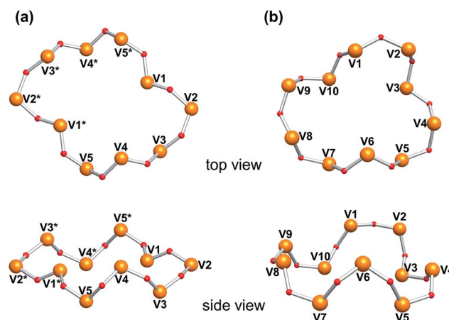
Fig. 3 Comparison of the \text{V}_{10}\text{O}_{10} rings in (a) Co2 and (b) Co3.
