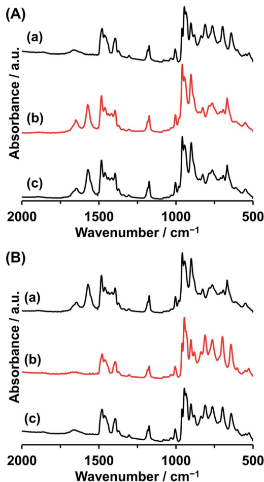
Fig. 2 (A) IR spectra of (a) Co2, (b) Co2 treated with 1.0 equiv. of \text{Co}(\text{OAc})_2 , and (c) Co3. (B) IR spectra of (a) Co3, (b) Co3 treated with 5.0 equiv. of \{\text{Et}_4\text{N}\}[\text{VO}_3] , and (c) Co2.
