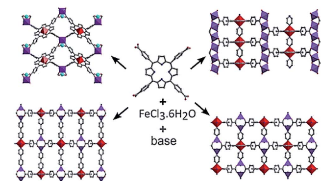
Scheme 16 The CPs obtained by the solvothermal reaction of \text{Fe}(\text{III}) chloride with tetrakis(4-carboxyphenyl)-Pp in the presence of different bases. [Reprinted with permission from ref. 212. Copyright 2015, American Chemical Society.]
