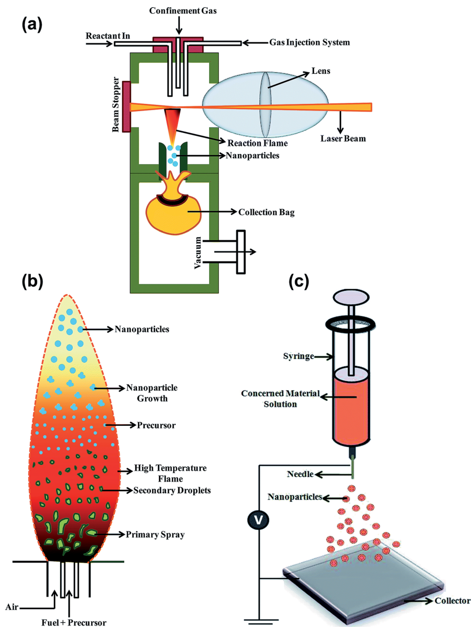
Fig. 10 Schematic diagrams of (a) laser pyrolysis, (b) flame spray pyrolysis and (c) an electro-spraying technique for the synthesis of nanoparticles. 80
