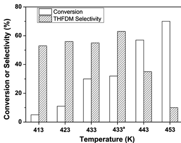
Fig. 4 Effect of temperature on the conversion of glucose to THFDM. a Repeated test for the temperature at 433 K. Reaction conditions: Nb 2 O 5 -FP (40 mg), Ru/SiO 2 -TM (30 mg), glucose aqueous solution (3 mL, glucose 1 mmol), cyclohexane (6 mL), H 2 (4 MPa), 433 K, 4 h.
