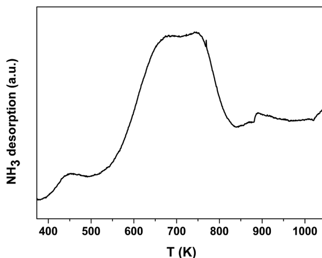
Fig. 7 \text{NH}_3 -TPD profiles of \text{Nb}_2\text{O}_5\text{-FP} .
