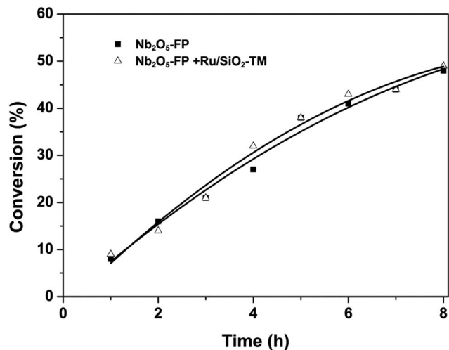
Fig. 2 Conversion–time profiles of glucose dehydration to HMF and glucose conversion to THFDM. Reaction conditions: Nb 2 O 5 -FP (40 mg), glucose aqueous solution (3 mL, glucose 1 mmol), cyclohexane (6 mL), H 2 (4 MPa), 433 K. \Delta : Ru/SiO 2 -TM (30 mg).
