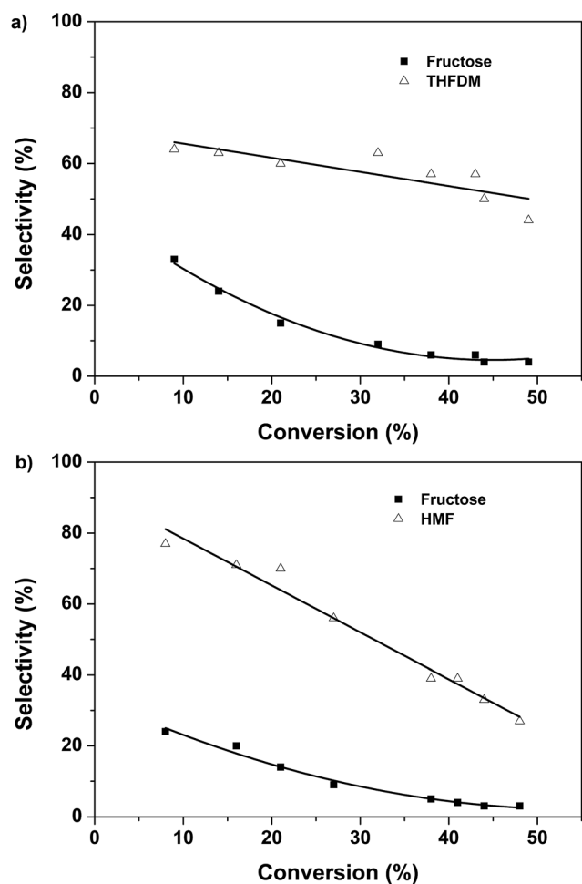
Fig. 3 Products selectivity versus glucose conversion over (a) Nb 2 O 5 -FP and Ru/SiO 2 -TM, (b) Nb 2 O 5 -FP. Reaction conditions: Nb 2 O 5 -FP (40 mg), glucose aqueous solution (3 mL, glucose 1 mmol), cyclohexane (6 mL), H 2 (4 MPa), 433 K. Ru/SiO 2 -TM (30 mg) for (a).
