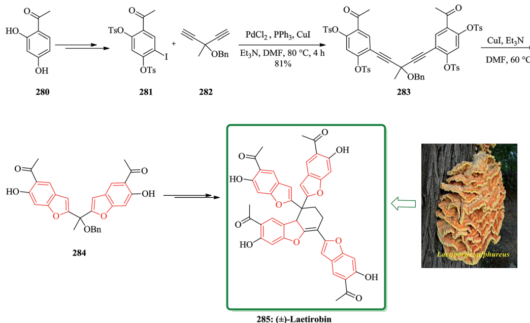
Scheme 61 Total synthesis of ( \pm )-laetiropin 285.
