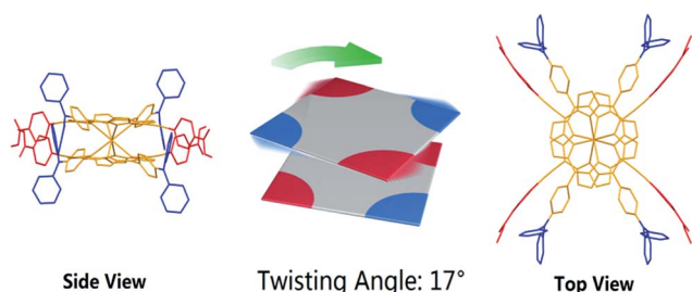
Fig. 2 The simulated molecular structure of HTb(DADAPor) 2 with a twisted octupolar cuboid skeleton and the group point of D_2 .
